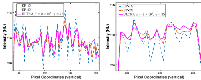
Fig. 11. Vertical (left) and horizontal (right) profiles of chest reconstructions (plotted from the central axial slice) for the PWLS-EP and PWLS-ULTRA methods. The profile locations are shown in green lines in Fig. 7.
